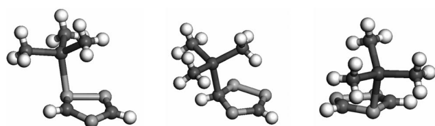
Figure 8. Calculated structures of (trimethylstannyl)-1,2,4-triphosphole isomers 9a (left), 9b (middle) and 9c (right). The CCSD(T)/LANL2DZ+2pol relative energies [kcal mol −1 ] of the three minima are 9a : 0.0, 9b : 3.1, and 9c : 1.2.
