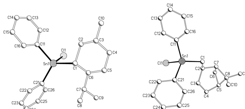
Figure 2. Molecular structures of (1 R )-(-)-menthyldiphenyltin chloride [( R )- 7b , left] and (-)- cis -myrtanyldiphenyltin chloride ( 7c , right) in the solid state.
