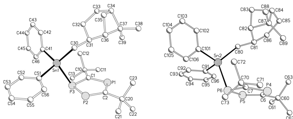
Figure 5. Molecular structure of the two diastereomers 2d ( SS , left) and 2d ( RS , right) in the solid state. Hydrogen atoms have been omitted for clarity.
