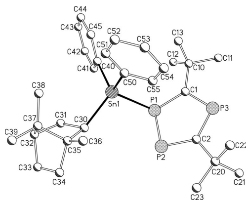
Figure 3. Molecular structure of one of the enantiomers of racemic exo -derivative 2a in the solid state. Solvent molecules and hydrogen atoms have been omitted for clarity.
