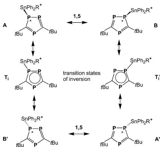
Scheme 5. Diastereomeric ground states ( A and B ) at equilibrium and inversion transition states ( \text{T}_i ) of 1-(triorganylstannyl)-1,2,4-triphosphole derivatives 2 .
