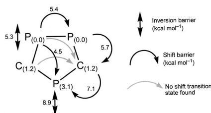
Figure 9. Shift-barrier calculation results [kcal mol −1 ] for 9 .
