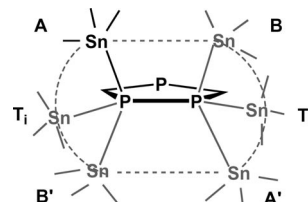
Figure 7. Cyclic rocking mode of the mobile stannyl group in front of the \text{P}_2 -edge of 1-(triorganylstannyl)-1,2,4-triphospholes 2 .
