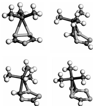
Figure 11. Calculated transition states T_s of suprafacial P–P (top) and P–C (bottom) stannyl group shifts for 9 .
