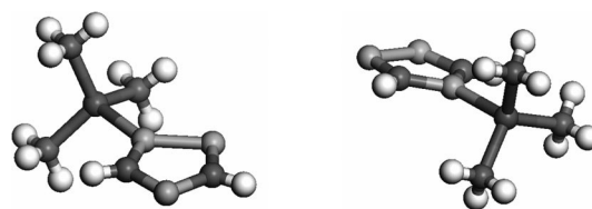
Figure 10. Calculated ring inversion transition states T i for 9a (left) and 9c (right).
