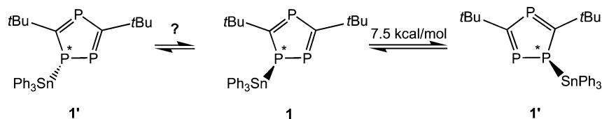
Figure 1. [1,5]-Sigmatropic shift of the \text{SnPh}_3 group of 1 .
